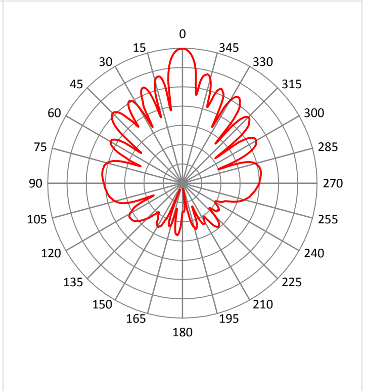
Elevation @ 5.8GHz
