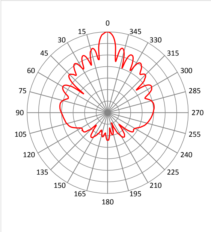
Azimuth @ 5.8GHz
